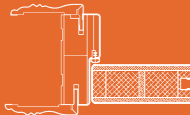
Construction of the door unit assembly
